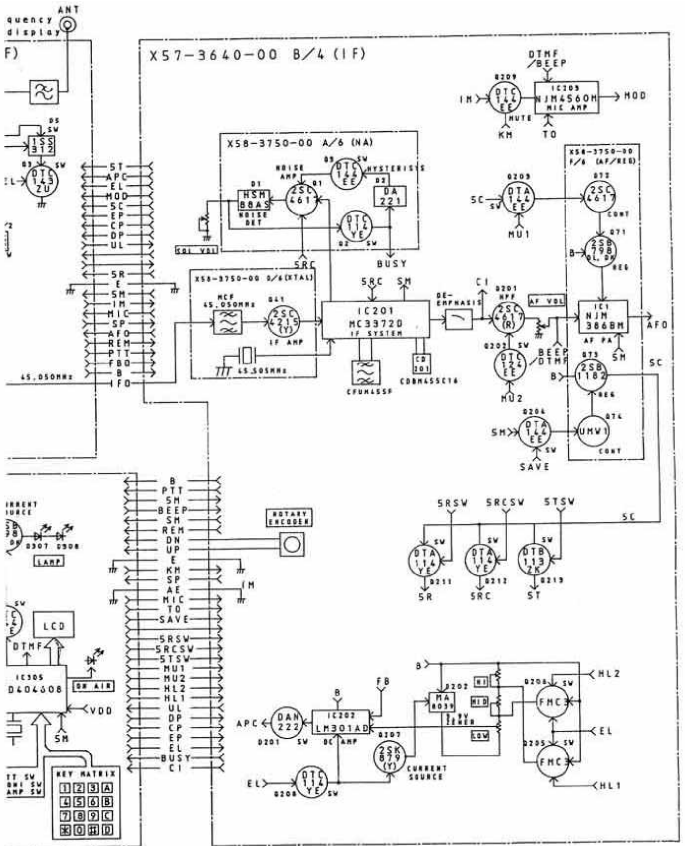
TH-F27 BLOCK DIAGRAM
